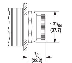
Selector Push Button Shipping Wt. 6 oz (0.17 kg)
