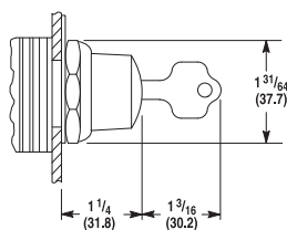
Key Operated Selector Switch Shipping Wt. 12 oz (0.34 kg)
