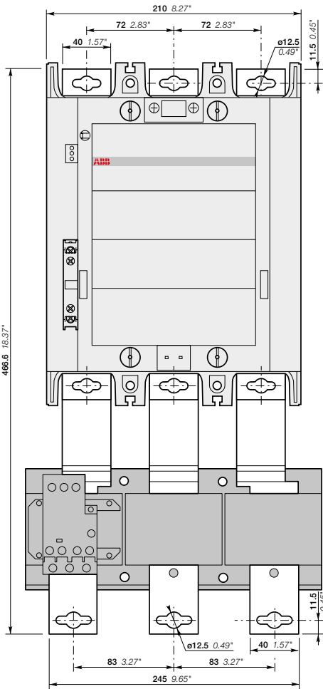
AF580 and AF750-30-11 + E800DU electronic O/L relay
