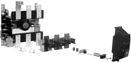
Typical NEMA Size 6 Contactor (exploded view)
