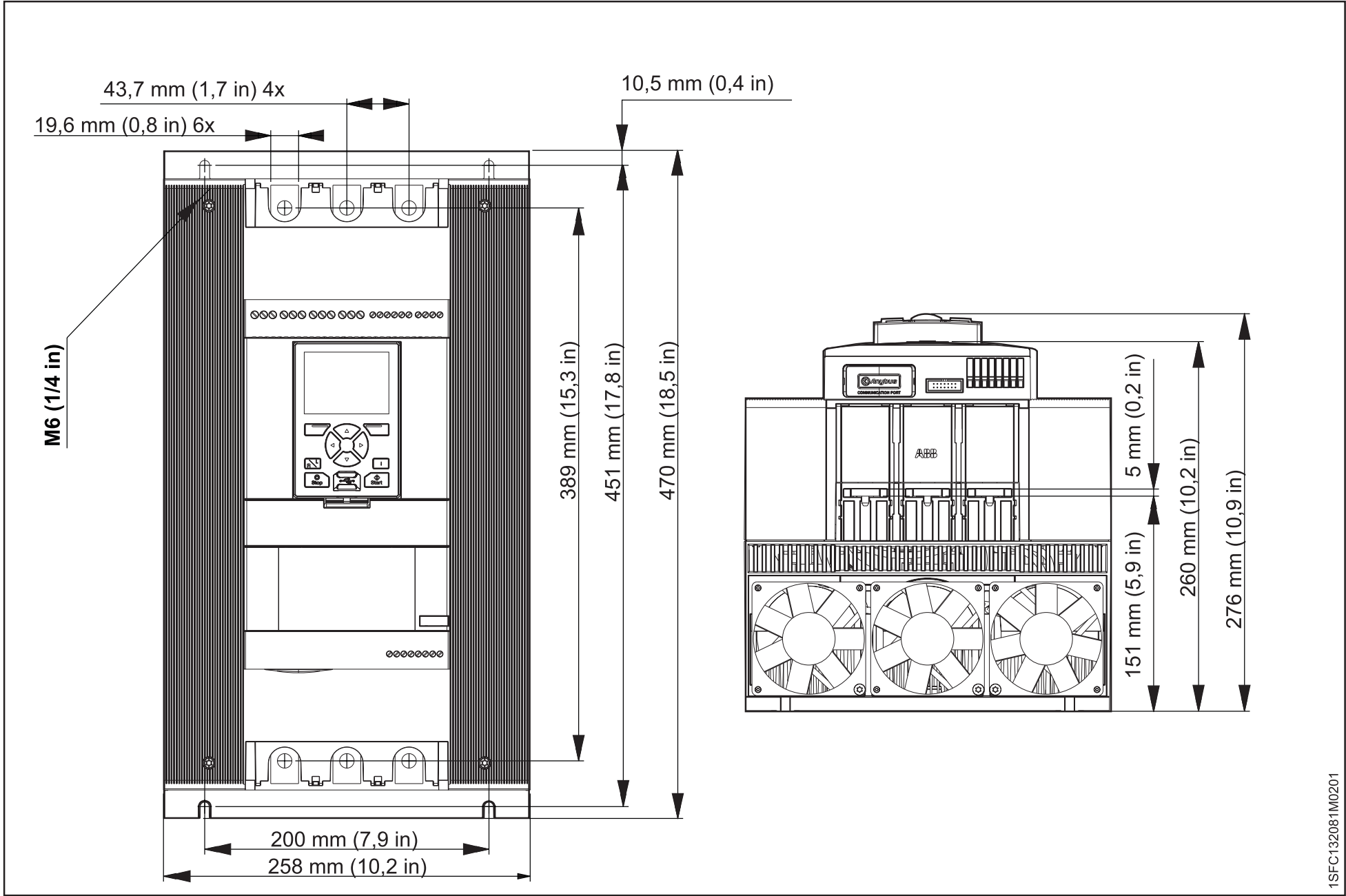
Dimensions PSTX210..370
