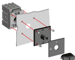
Screw mounting S00267A
