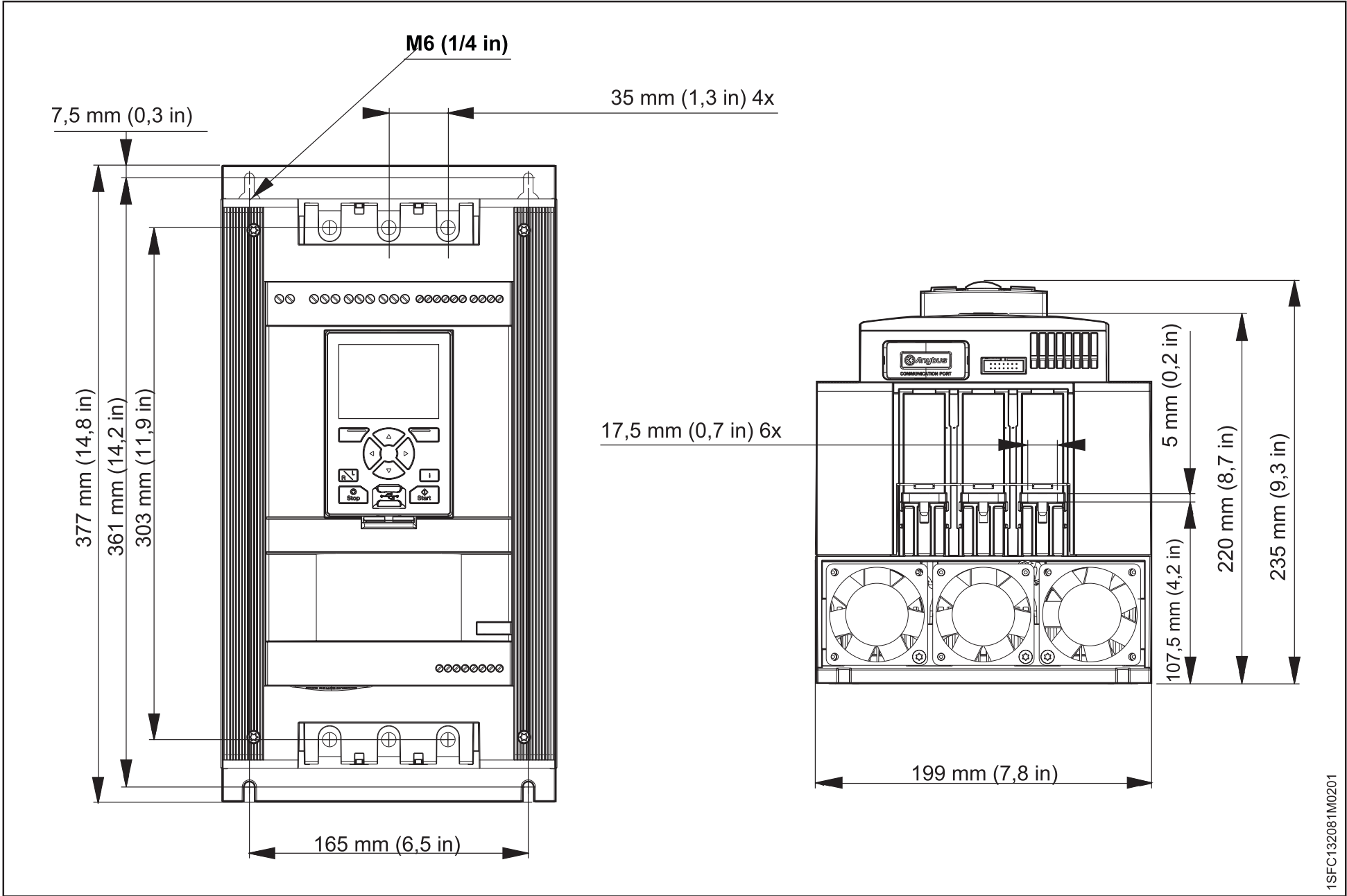
Dimensions PSTX142...170
