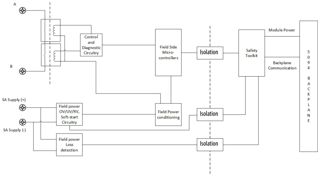
5094-0W4IS and 5094-0W4ISXT Functional Block Diagram
