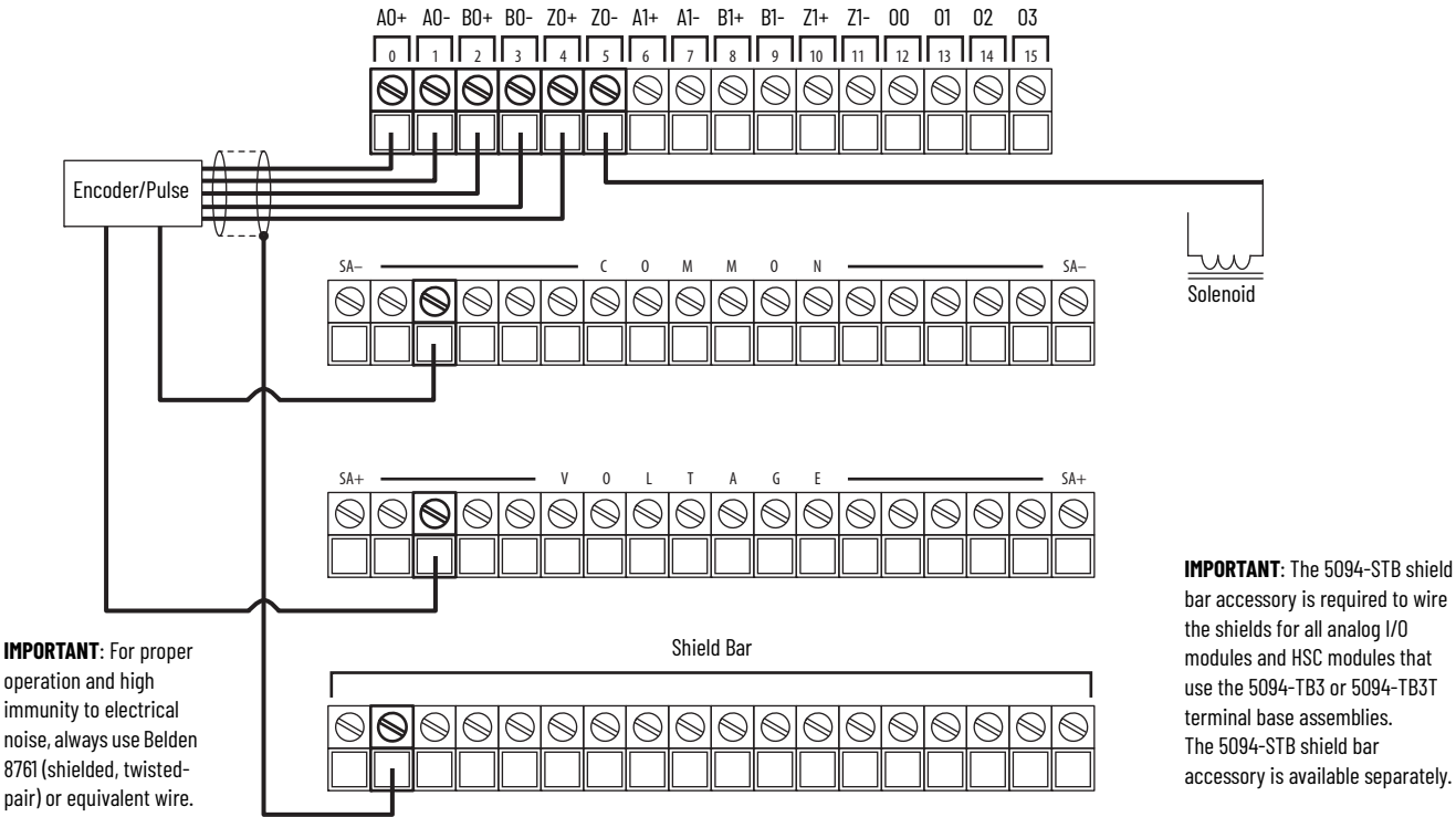
5094-HSC and 5094-HSCXT Wiring Diagram - Differential Encoder
