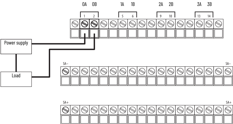
5094-0W4IS and 5094-0W4ISXT Wiring Diagram
