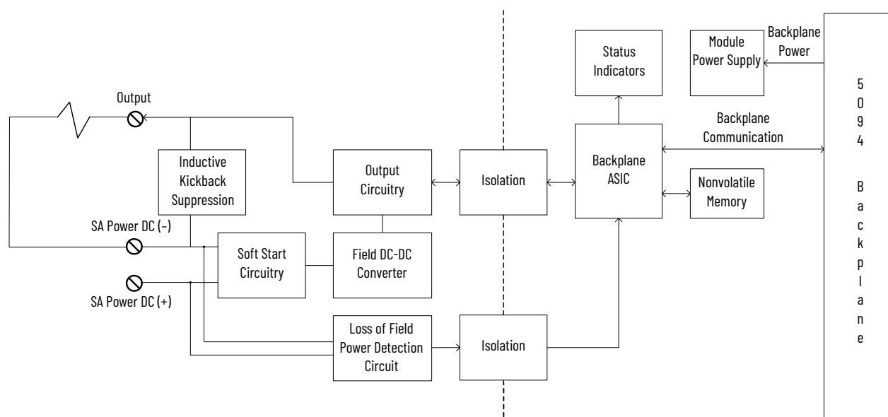
5094-OB16 and 5094-OB16XT Functional Block Diagram
