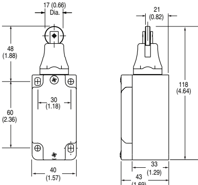
Roller Plunger
