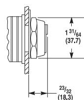
Coin Slot Selector Switch Shipping Wt. 6 oz (0.17 kg)
