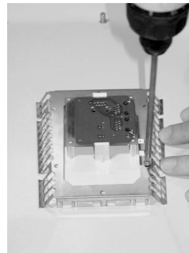
9. Align screw openings of the stainless steel bracket in the platform holes with screws. Screw six (6) screws in place.
