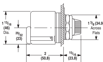
Type J Potentiometer Unit
