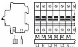
SZ-PSB 58 N SK 0100 Z96 SZ-PSB 60 N 1-pole + NA with 4 phases or 3 phases + N
