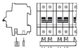
SZ-PSB 92 N SK 0099 Z 96 2-pole + auxiliary switch with 2 phases 1-pole + NA + auxiliary switch, with 2 phases or 1 phase + N + auxiliary switch
