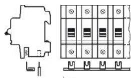
SZ-KS 3/39 N SK 0095 Z 96 SZ-KS 4/39 N 1-pole + aux.sw.. with 1 phase
