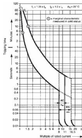
S 220-K 0.2 ... 8 A K 40 ... 63 A
