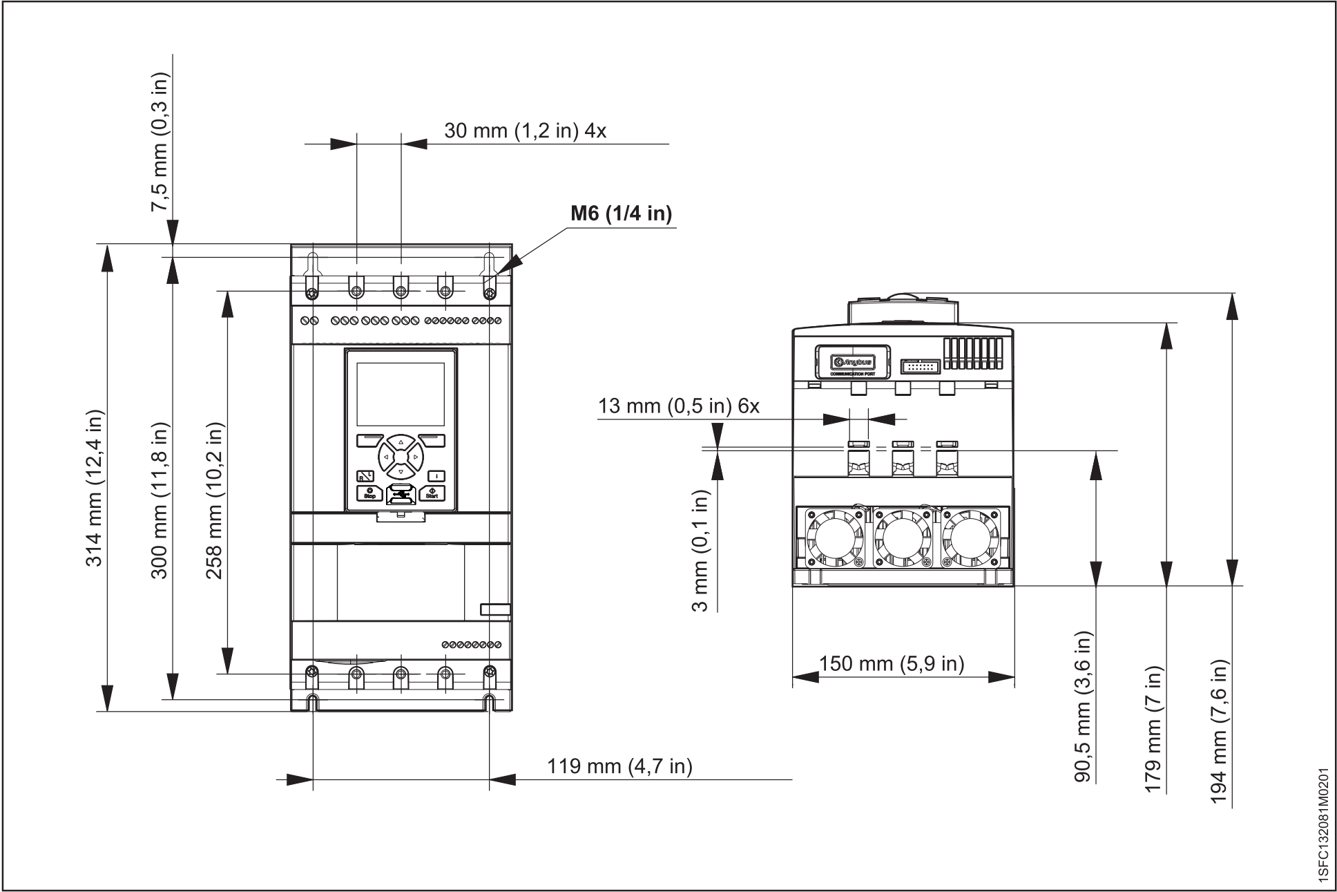
Dimensions PSTX30...105
