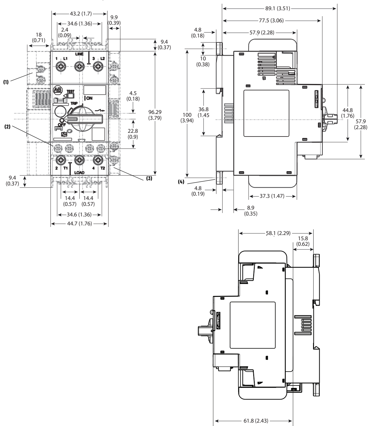
Figure 3 - Molded Case Circuit Breaker, Cat. No. 14OUT-D7...
