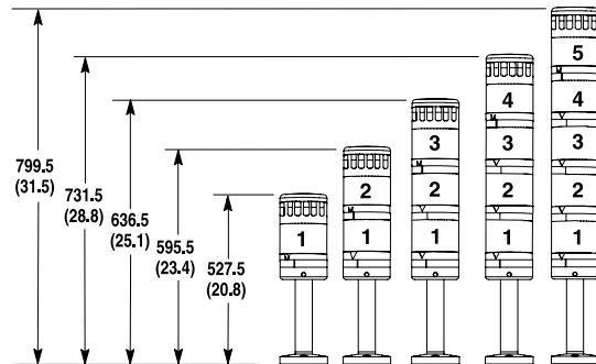
60 cm Pole Mount Base (SPM60)
