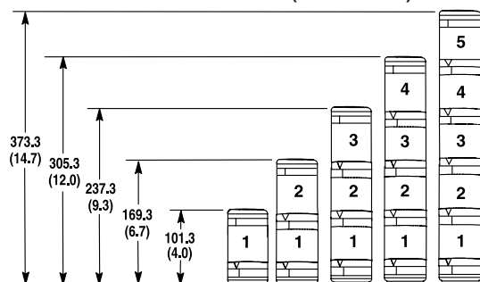
10 cm Pole Mount Base (PM10, SPM25)
