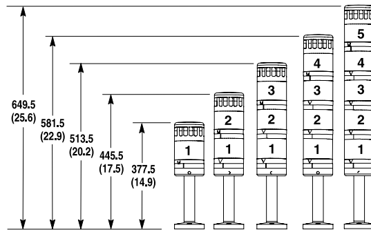
Tube Mount Base (TM)
