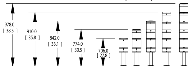
60 cm Pole Mount Base (SPM60)
