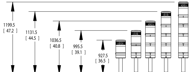
80 cm Pole Mount Base (SPM80)
