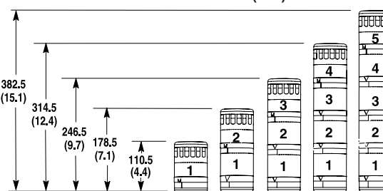
Tube Mount Base (TM)
