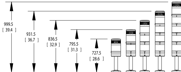
60 cm Pole Mount Base (SPM60)
