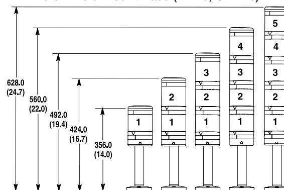
Tube Mount Base (TM)
