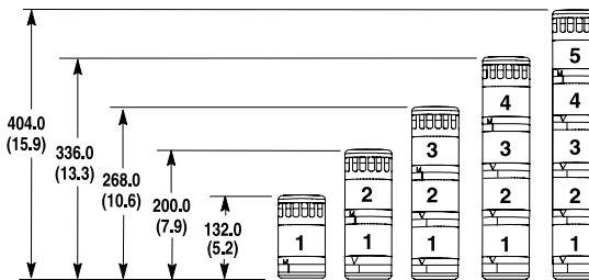
Tube Mount Base (TM)
