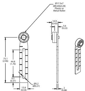
Cat. No. 440P-CAL_ , -CRR_ , -MAL_ , and -MRR_ Adjustable Lever (Plastic & Metal Roller)
