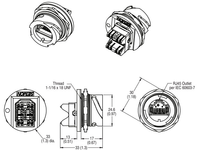
Female Receptacle
