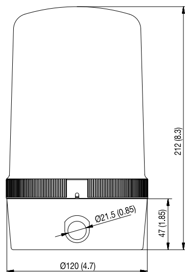
120 mm Beacon Surface Mount
