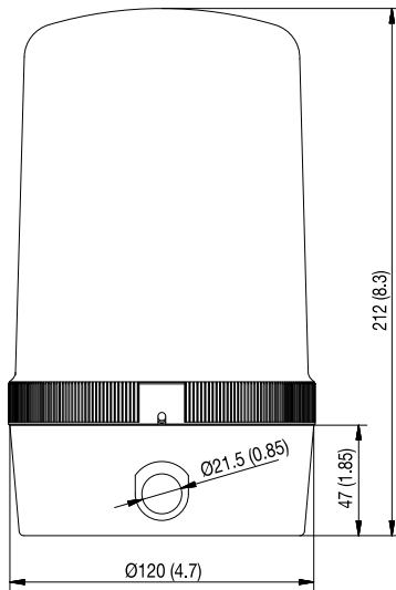
120 mm Beacon Tube Mount
