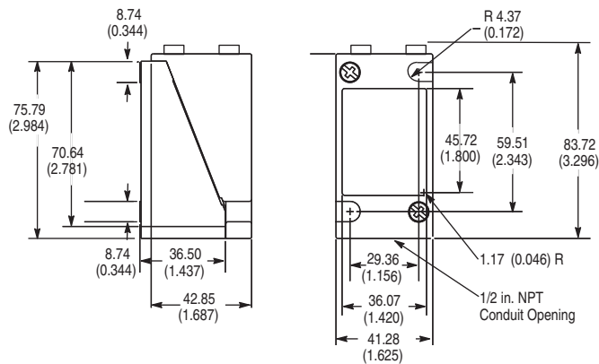
Switch Body
