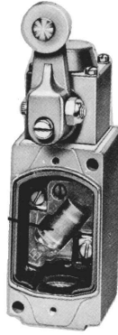
802R-AF (cover removed) with 802T-W1 Lever
