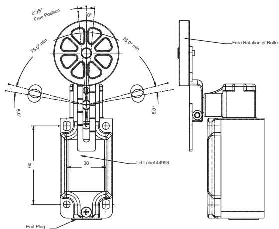
Rubber Roller
