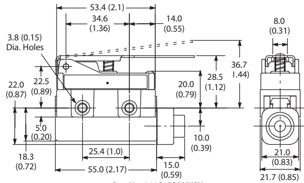
Cat. No. 802B-SSAHXSX
