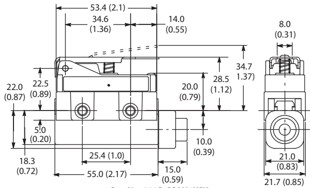
Cat. No. 802B-SSAH1XSX
