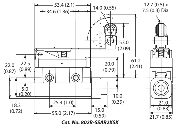
Cat. No. 802B-SSAR2XSX
