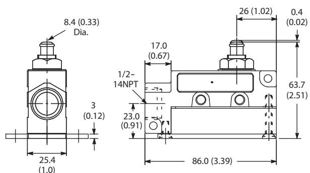
Cat. No. 802B-PFABXSX
