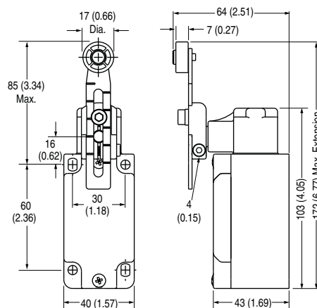
Adjustable Lever
