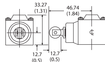
Z-36622 Side Push Vertical Roller Head Shipping Wt. 0.12 kg (4.25 oz)
