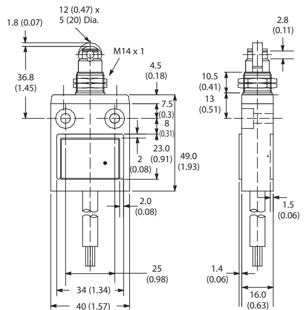
Top Push Roller Panel Mount
