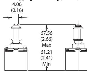
Adjustable Top Push Rod Head for Cat. No. 802T-BAT
