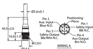
4-pin Micro Quick Disconnect
