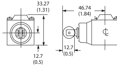
Cat. Nos. 802T-KT & 802T-K1T Side Push Roller Head
