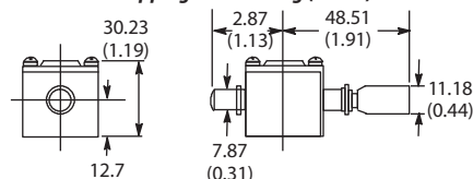
802T-CM Maintained Side Push Rod Head Shipping Wt. 4.5 oz (0.128 kg)
