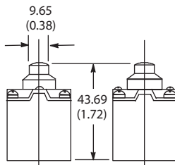
Cat. No. 802T-BT Top Push Rod Head
