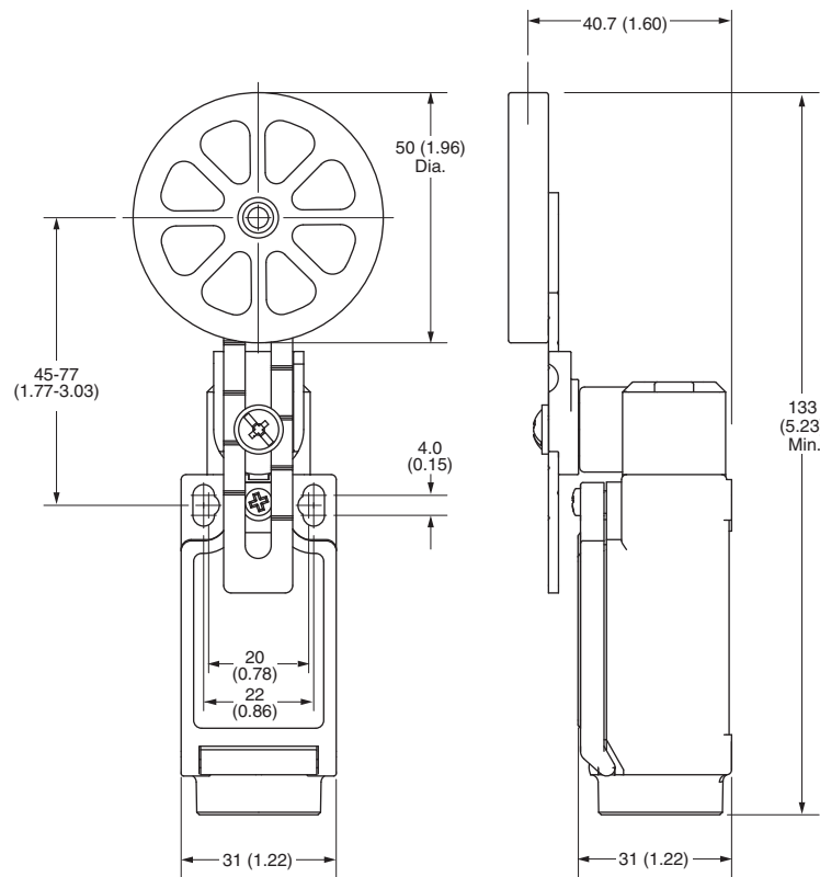
Rubber Roller
