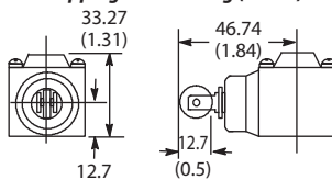
802T-K Side Push Roller Head Shipping Wt. 0.128 kg (4.5 oz)
