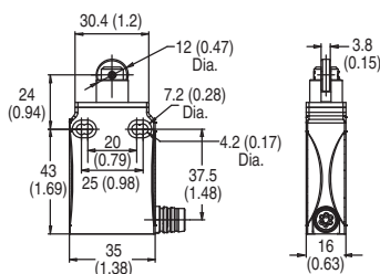
Roller Plunger
