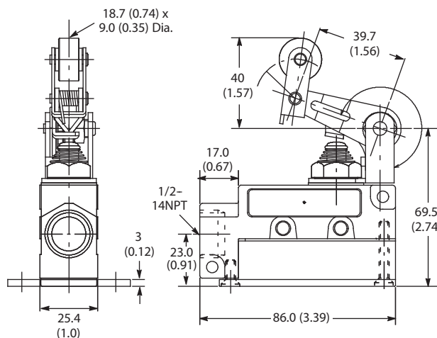
Cat. No. 802B-PFAR2XSX
