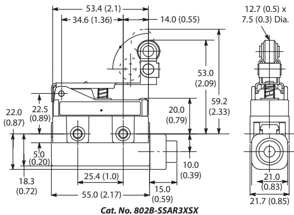
Cat. No. 802B-SSAR3XSX
