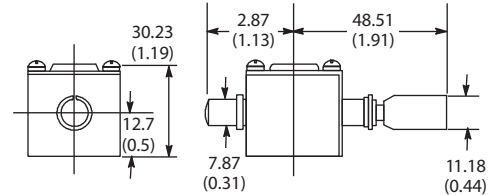
Cat. No. 802T-CT Side Push Rod Head
