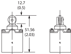
Cat. No. 802T-DT Top Push Roller Head
