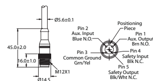
5-pin Micro Quick Disconnect
