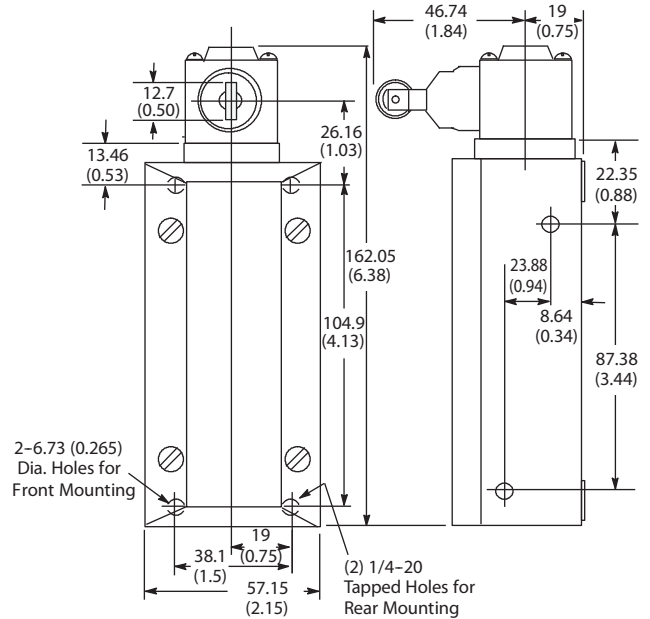
Bulletin 802XR Side Push Roller Type Approximate Shipping Wt. 0.9 kg (2 lb)
