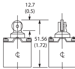
Z-36618 Top Push Roller Head Shipping Wt. 0.12 kg (4.25 oz)
