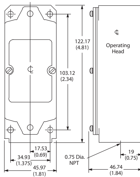
NonPlug-in Switch
