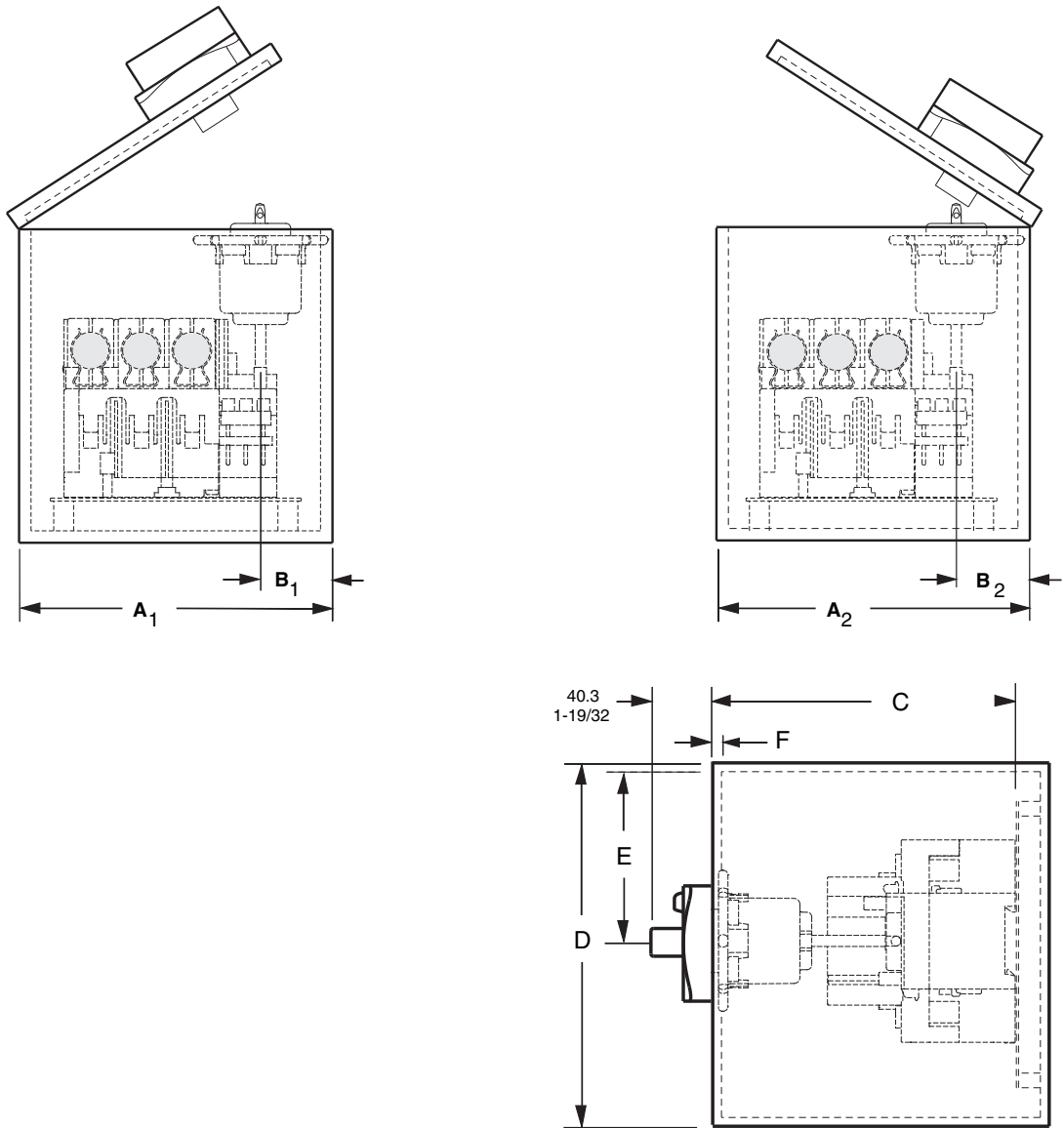
ENCLOSURE INSTALLATION DIMENSIONS
