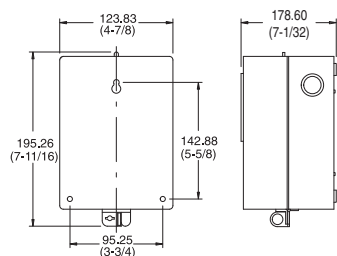
Cat. No. 700-N31, Type 1 Enclosure for Bulletin 700-P, -RTC Relays Approximate Shipping Weight: 1.26 kg (2.8 lb)
