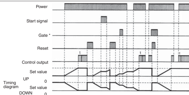
Output Mode A-3 Power ON Delay 2 (Timer does not reset when power comes ON)
