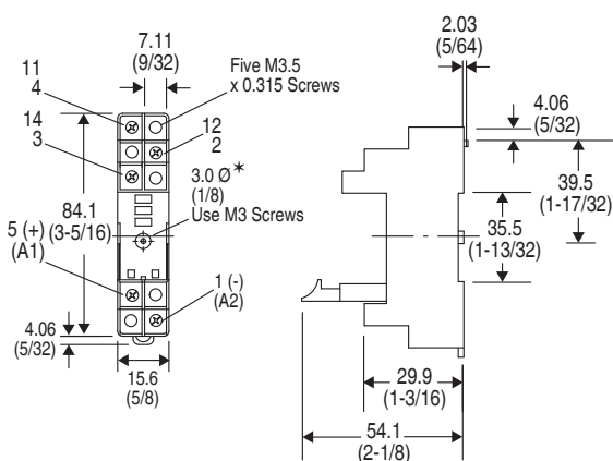
Bulletin 700-HNC41 SPDT Contact Approximate Dimensions
