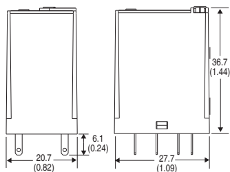
Bulletin 700-HC Relay (Two-Pole)
