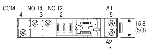
Cat. No. 700-HN221
