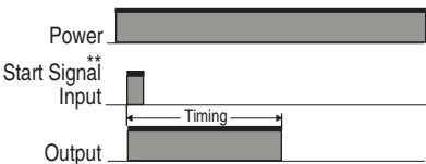
Output Mode F: Cumulative (Timer does not reset when power comes ON)
