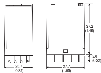
Bulletin 700-HC Relay (Four-Pole)
