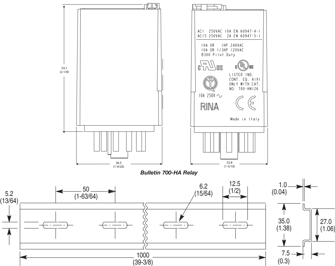
Cat. No. 199-DR1 DIN Mounting Rail Series B Cat. No. 199-DR4 DIN Mounting Rail Series B Has No Mounting Holes
