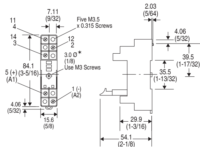
Cat. No. 700-HN121
