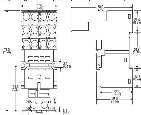
Cat. No. 700-HN128★
