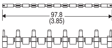
Bulletin 700-TBJ08_ 8-Way Jumper
