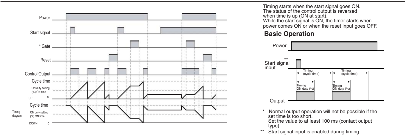
Output Mode S: Stop Watch (Timer resets when power comes ON)
