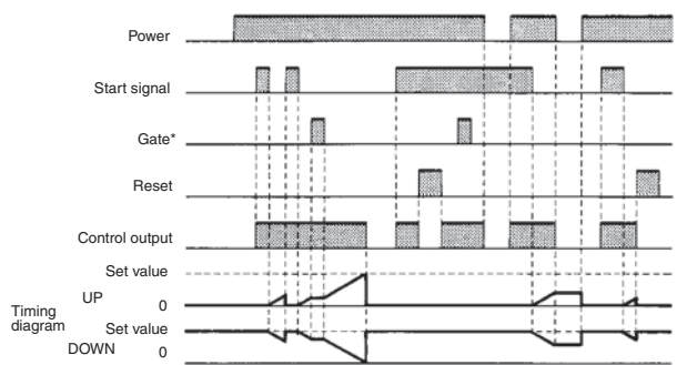
Output Mode E: Interval (Timer resets when power comes ON.)
