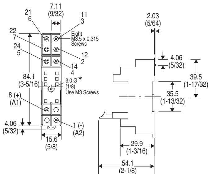
Cat. No. 700-HN122
