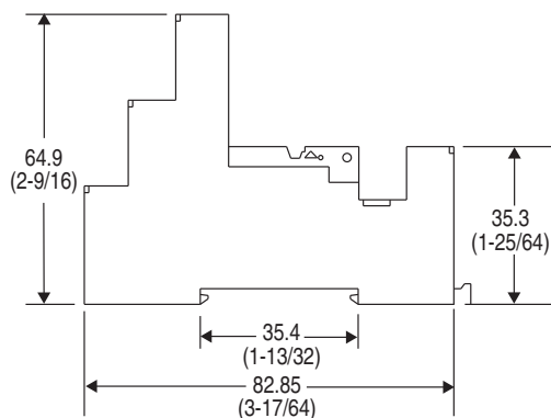
Cat. No. 700-HN221
