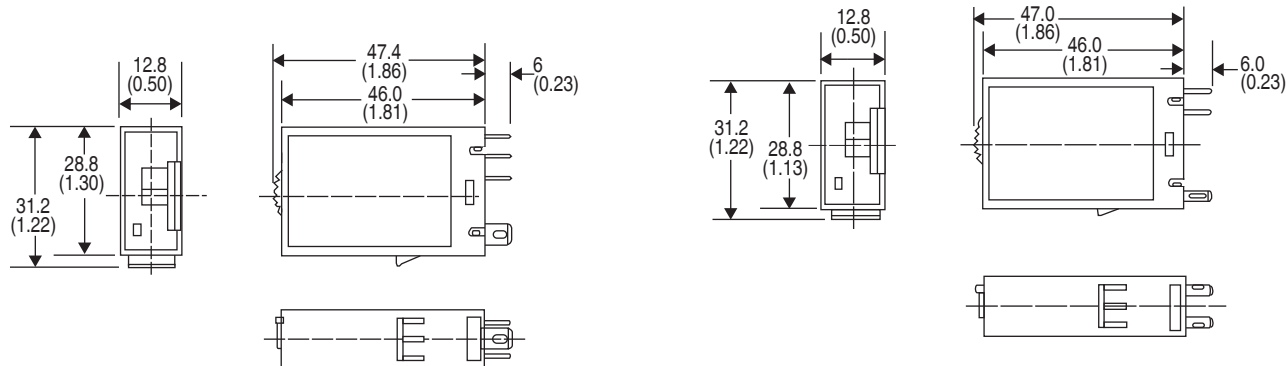
Bulletin 700-HNC41 SPDT Contact Approximate Dimensions
