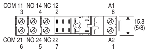
Cat. No. 700-HN222
