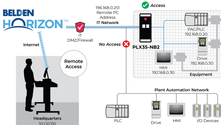
On-demand Secure Remote Access Application using the PLX35-NB2.
