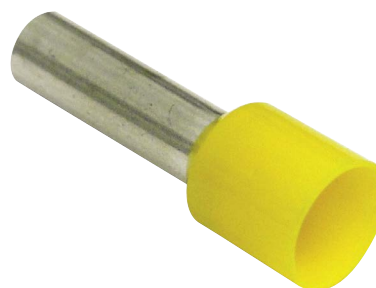
A cylindrical tube of tin-coated copper (with or without an insulated collar) that can be crimped onto the end of a wire.
