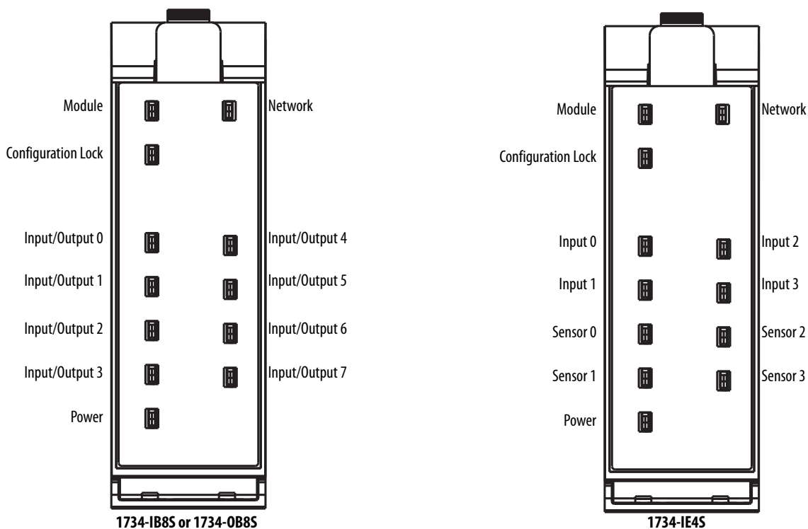
Figure 51 - Indicators Placement
