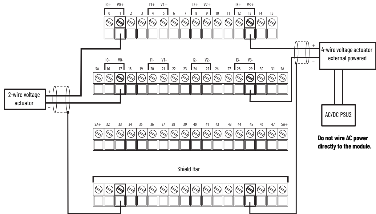
5094-OF4IHS and 5094-OF4IHSXT Wiring Diagram - 2- or 4-wire Voltage Actuator
