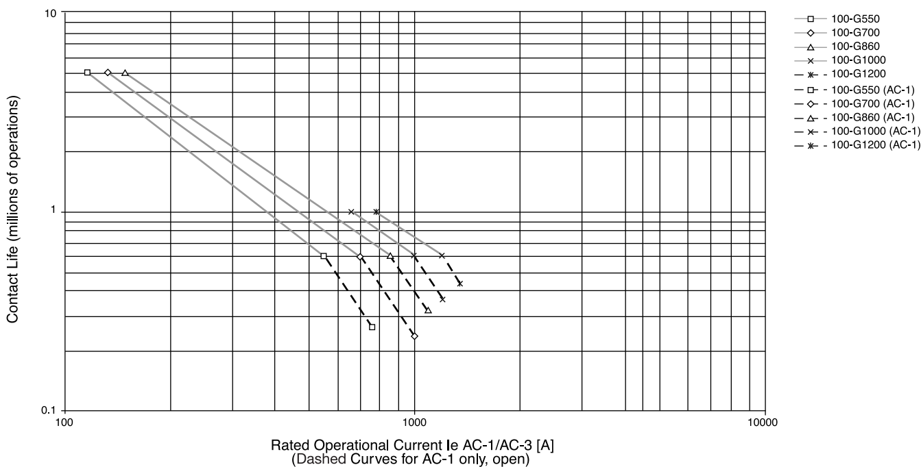
Figure 27 - AC-3 Switching of Running Three-phase Motors, U_e = 380 \dots 460V AC; AC-1 Non or Slightly Inductive Loads, Resistance Furnaces
