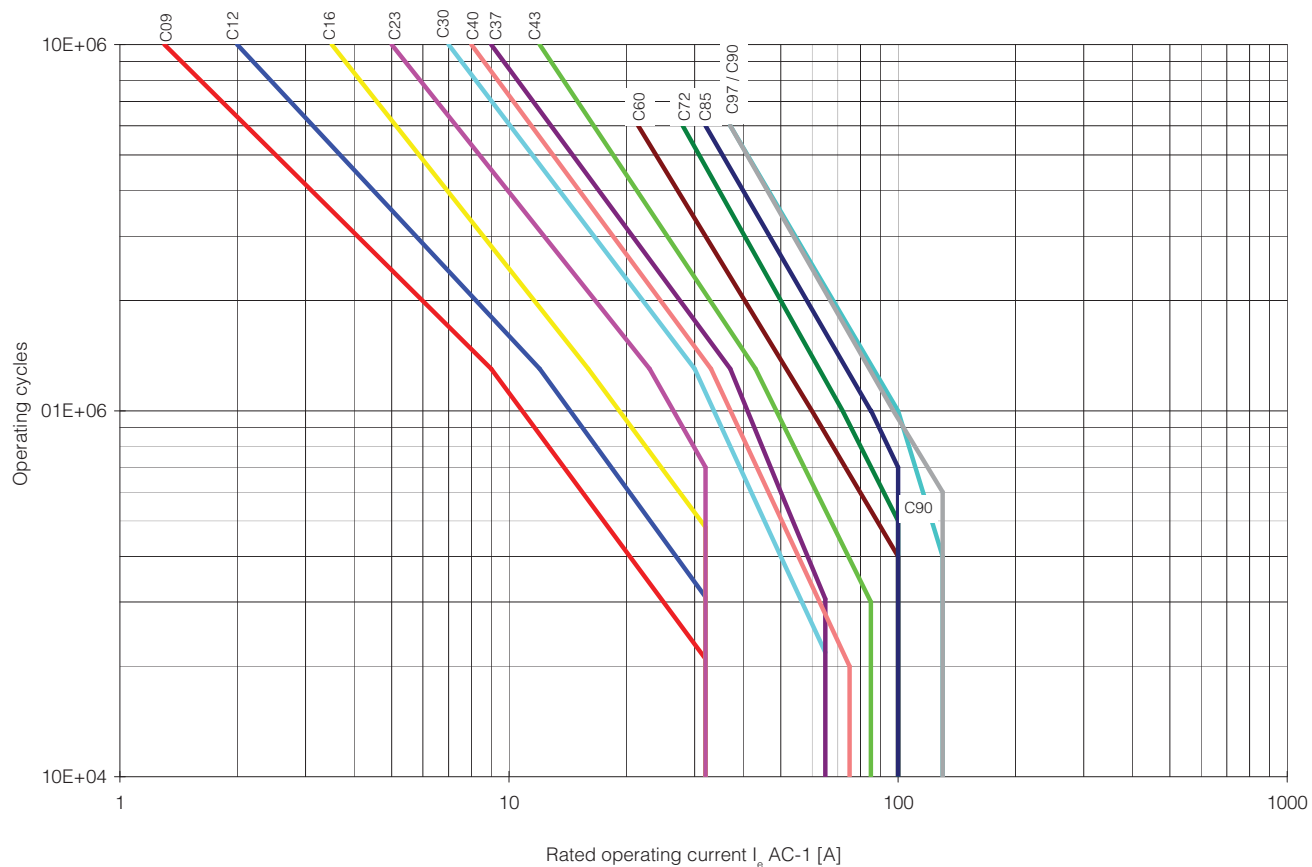
Figure 5 - AC-1, 40 °C Non- or slightly inductive loads, resistance furnaces; U_e = 230 \dots 690 \text{ V}
