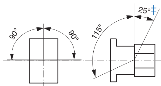
Figure 26 - Mounting Position, 100S-D Contactors
