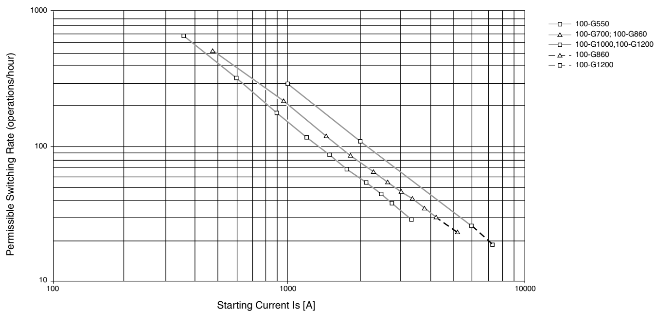
Figure 32 - Switching of Starting Motors (AC-2, and AC4) U_z = 380 \dots 460V AC; Starting Time t_{ed} = 1\text{ s} , ( < t_s )
