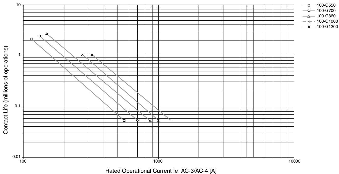
Figure 29 - AC-3 90% Switching of Running Motors, U_e = 380...460V AC; AC-4 10% Jogging
