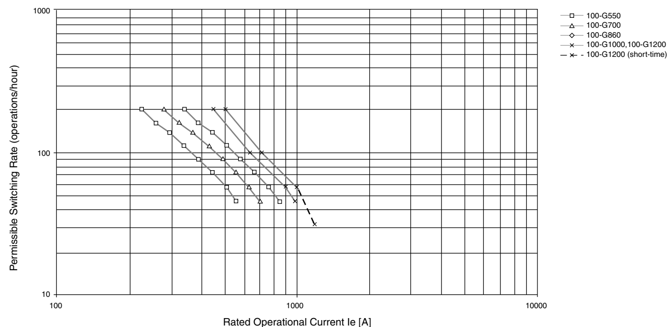
Figure 31 - Switching of Running Squirrel-cage Motors AC-3, U_e = 380...460V AC; Starting Time t_s = 1 s, Relative Running Time 40%
