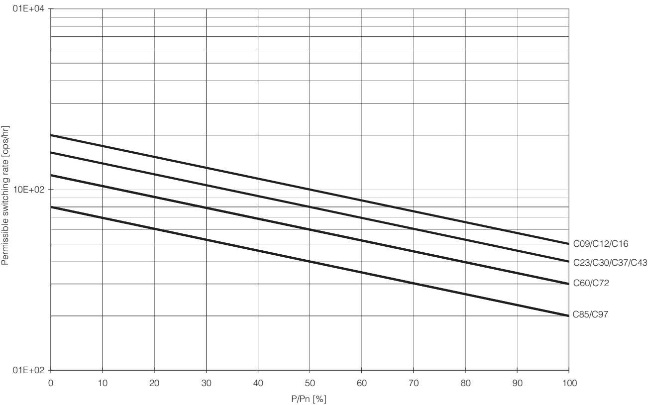
Figure 14 - AC-2, Stepping of slip-ring motors; U_e = 230 \dots 460V
