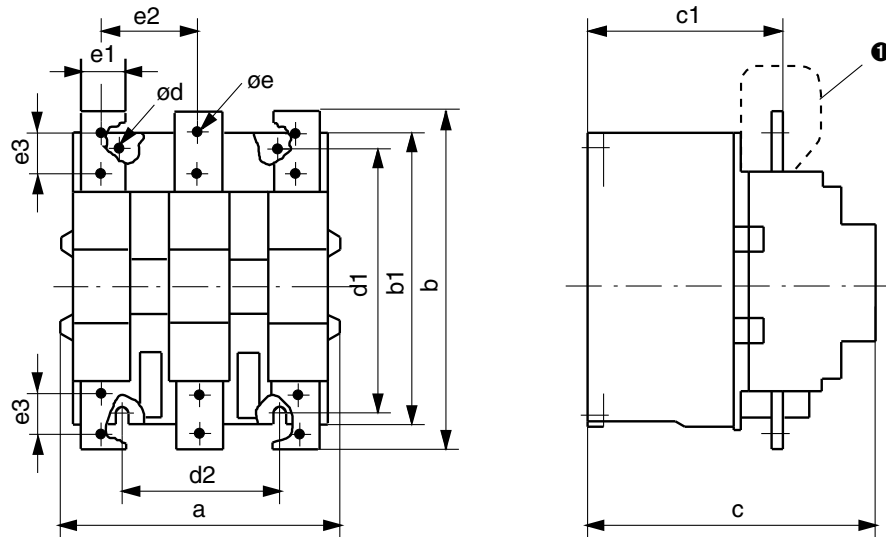
Figure 34 - Mounting Position
