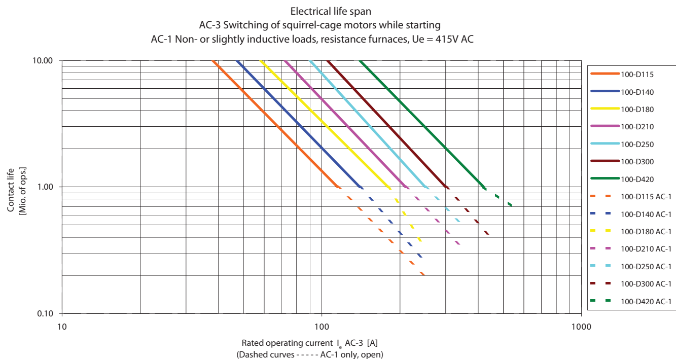
Figure 21 - AC-3, AC-1
