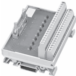
20-pin cable connector ON-state LED Narrow module for 24V: Cat. No. 1492-IFM20D24N 20-point LED module for 120V: Cat. No. 1492-IFM20D120, 20-pin cable connector LED Isolated module for 24V: Cat. No. 1492-IFM20DS24-4
