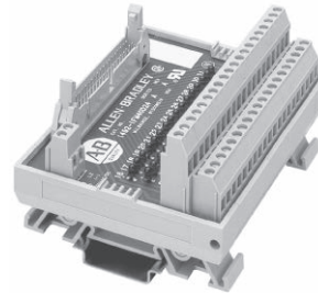
LED Indicating Extra Terminals For 20-point: Cat. No. 1492-IFM20D24-2, 1492-IFM20D24A-2, 1492-IFM20D120-2, 1492-IFM20D120A-2, 1492-IFM20D240-2, 1492-IFM20D240A-2 For 40-point: Cat. No. 1492-IFM40D24-2, 1492-IFM40D24A-2, 1492-IFM40D120-2, 1492-IFM40D120A-2
