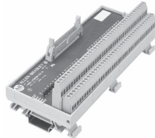
LED Indicating 4 Terminals For 20-point: Cat. No. 1492-IFM20DS24-4, 1492-IFM20DS120-4 For 40-point: Cat. No. 1492-IFM40DS24-4, 1492-IFM40DS24A-4, 1492-IFM40DS120-4, 1492-IFM40DS120A-4, 1492-IFM40DS240-4
