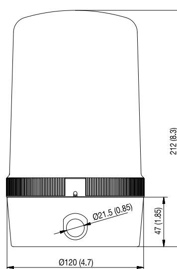
120 mm Beacon, Tube Mount
