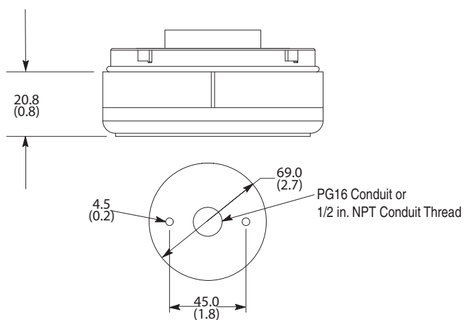
Surface-mount Base 855T-BSB or 855T-BCB
