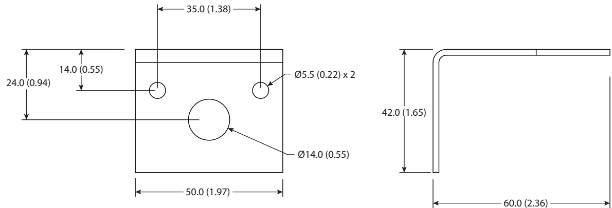
Catalog Number 855E-AVM Vertical-mount Bracket
