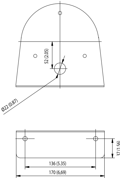
160 mm Beacon, Vertical Bracket
