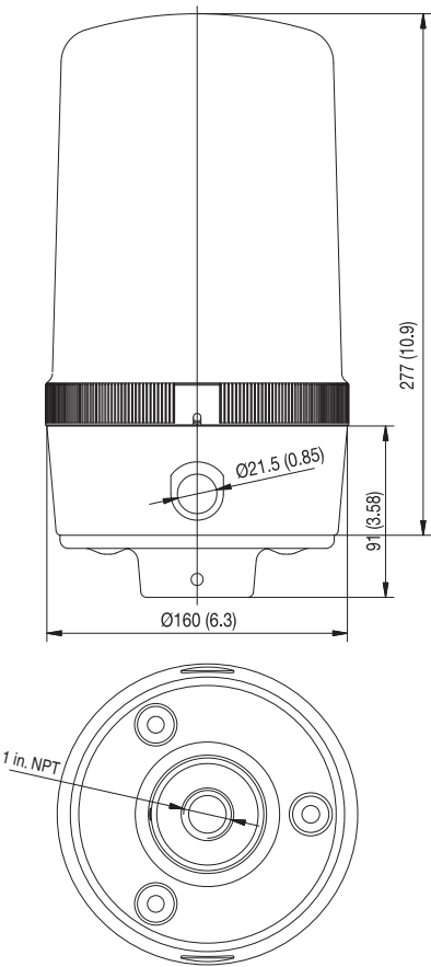
160 mm Beacon, NPT Conduit Mount
