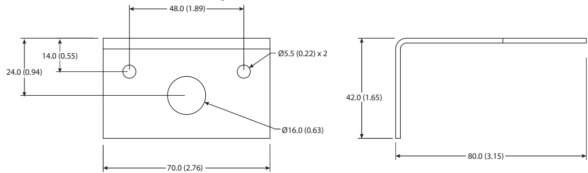
Catalog Number 855T-AVM Vertical Mount Bracket
