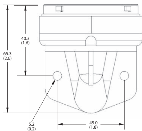
Vertical-mount Base
