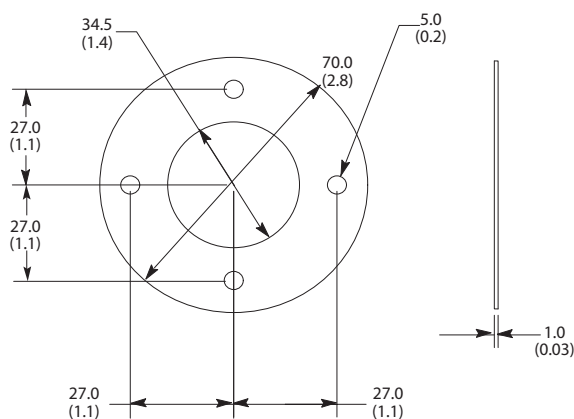
Vertical-mount Gasket
