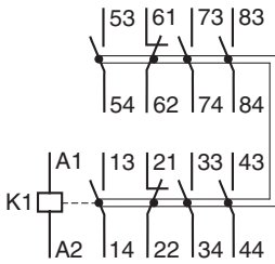
700S-CF620... 700S-CFB620...
