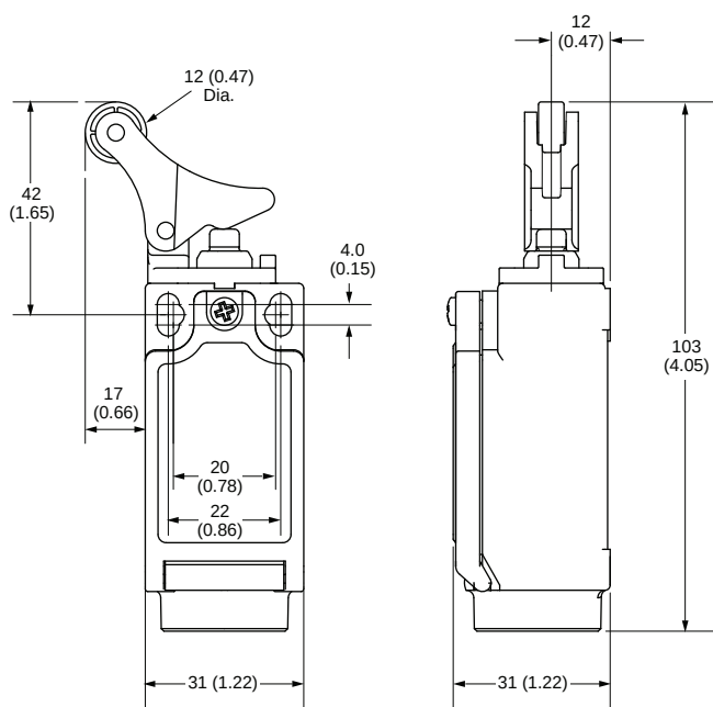
Offset Hinge
