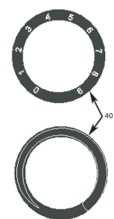
Anti-Rotation Washer
