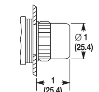
Round Push Button Illuminated Flush
