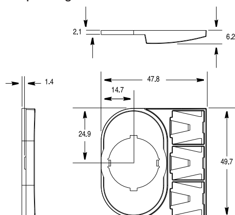
30 mm to 22.5 mm Hole Adapter
