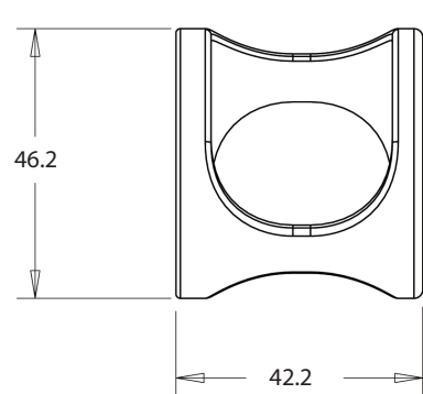
Protective Ring
