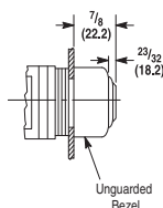
Square Backlit with Unguarded Bezel
