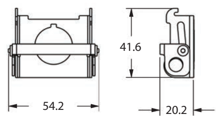
Momentary Mushroom Locking Attachment
