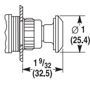
Round Push-Pull
