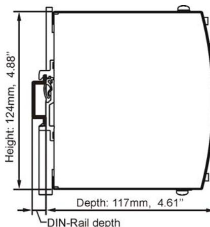
Fig. 22-2 Side view
