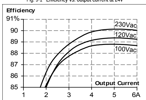
Fig. 9-1 Efficiency vs. output current at 24V
